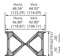
Center Pivot Horiz. Articulating Block
