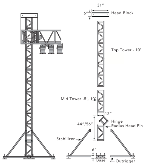
12" Tower Configuration
