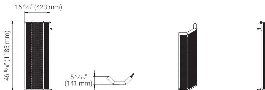
90° Compensator
