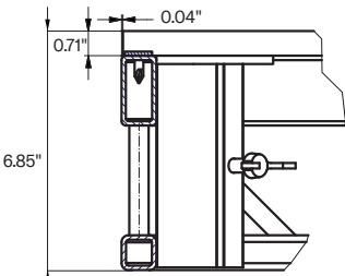
Cross section of profile
