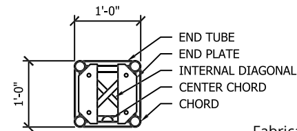
End View
