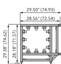
2-Way Corner Block
