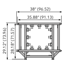
3-Way Corner Block
