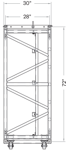
End View
